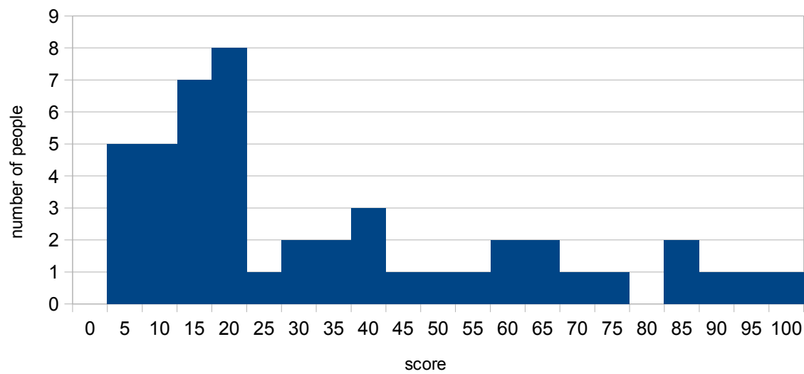
Quiz 2 histogram
