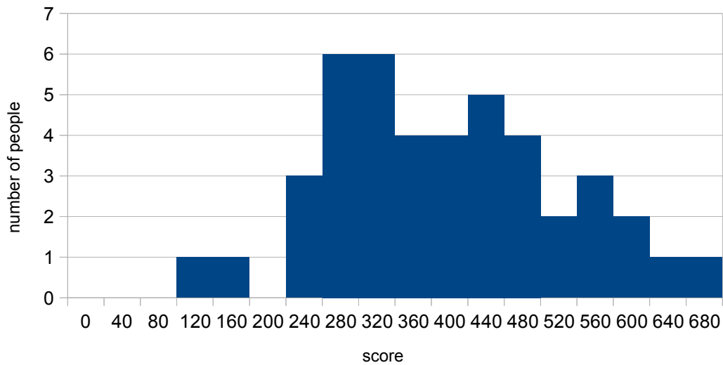
Histogram total
